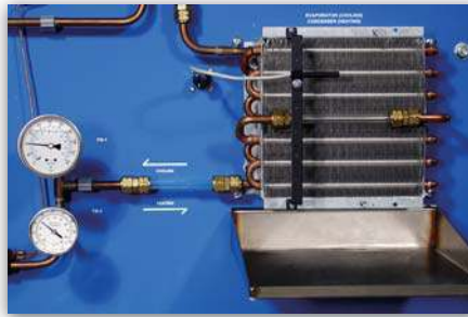
Evaporator Sight Glass and Instrumentation
