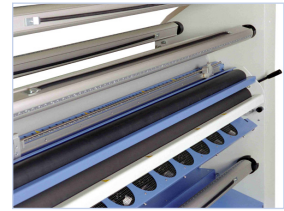
Flip-up pull rollers (62 Pro D)
